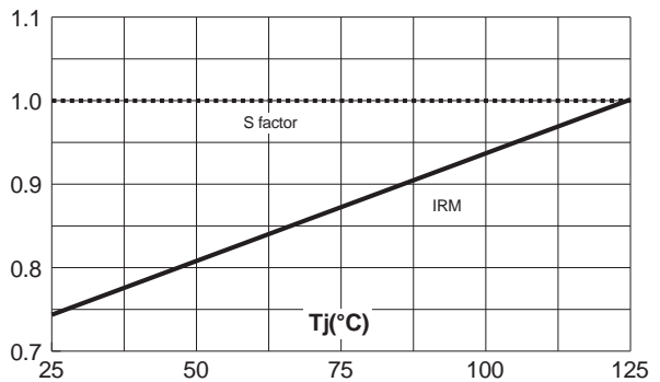
Fig. 6: Relative variation of dynamic parameters versus junction temperature (reference Tj = 125^{\circ}C ).
