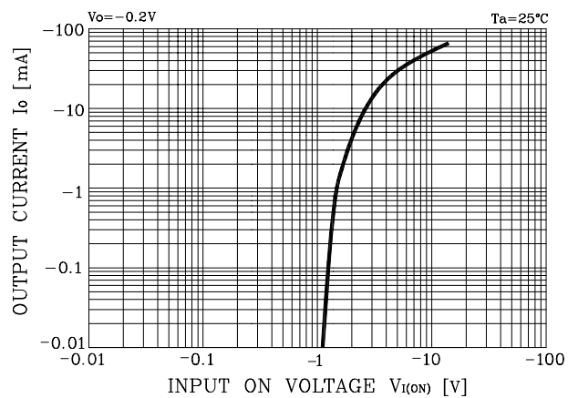
Fig. 1 I_O - V_{I(ON)}
