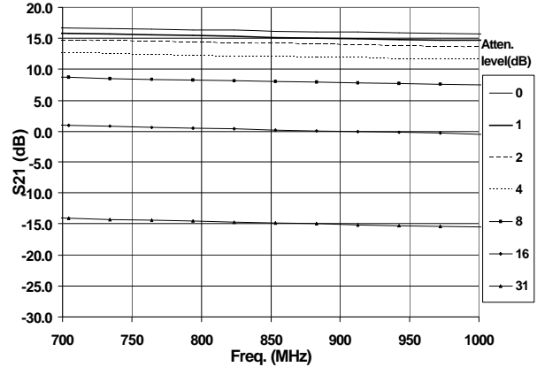
T=-40c Attenuation Error vs. Frequency
