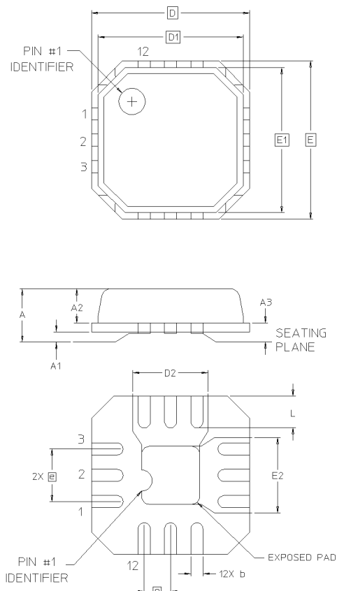
3 mm FQFP-N 12 Lead Anvll Singulated
