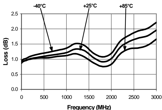
Typical Insertion Loss Variation at Temperature - Jx-J0
