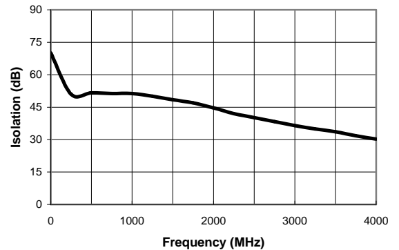
Isolation (dB) vs. Frequency
