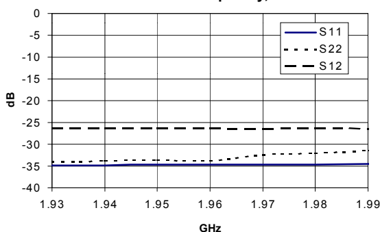
Input/Output Return Loss, Isolation vs. Frequency, T=25^{\circ}C
