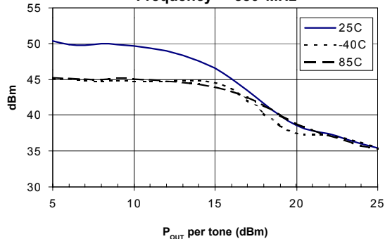
Third Order Intercept vs. Tone Power Frequency = 880 MHz
