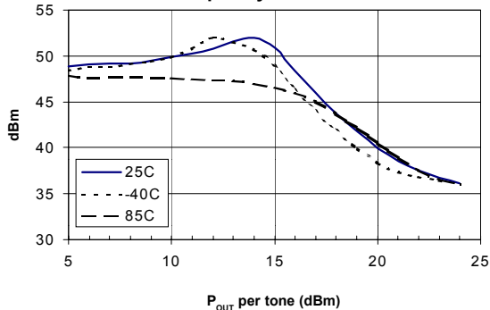
Third Order Intercept vs. Tone Power Frequency = 1.96 GHz
