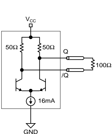
Figure 4. CML DC-Coupled
