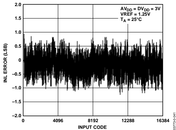
Figure 12. AD5390-3/AD5392-5 INL Plot
