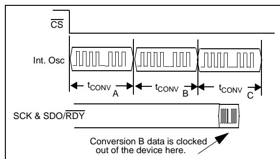
FIGURE 5-5: Most Current Continuous Conversion Mode Data.
