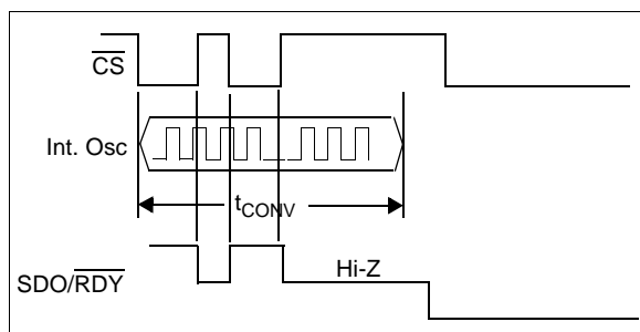
FIGURE 5-4: \overline{RDY} Functionality in Single Conversion Mode.
