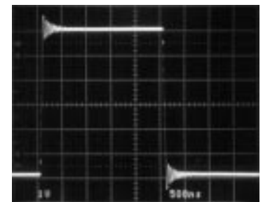
Large-Signal Transient, A_V = 1, C_L = 1000\text{pF}
