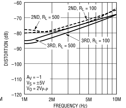
Distortion vs Frequency, A_V = -1
