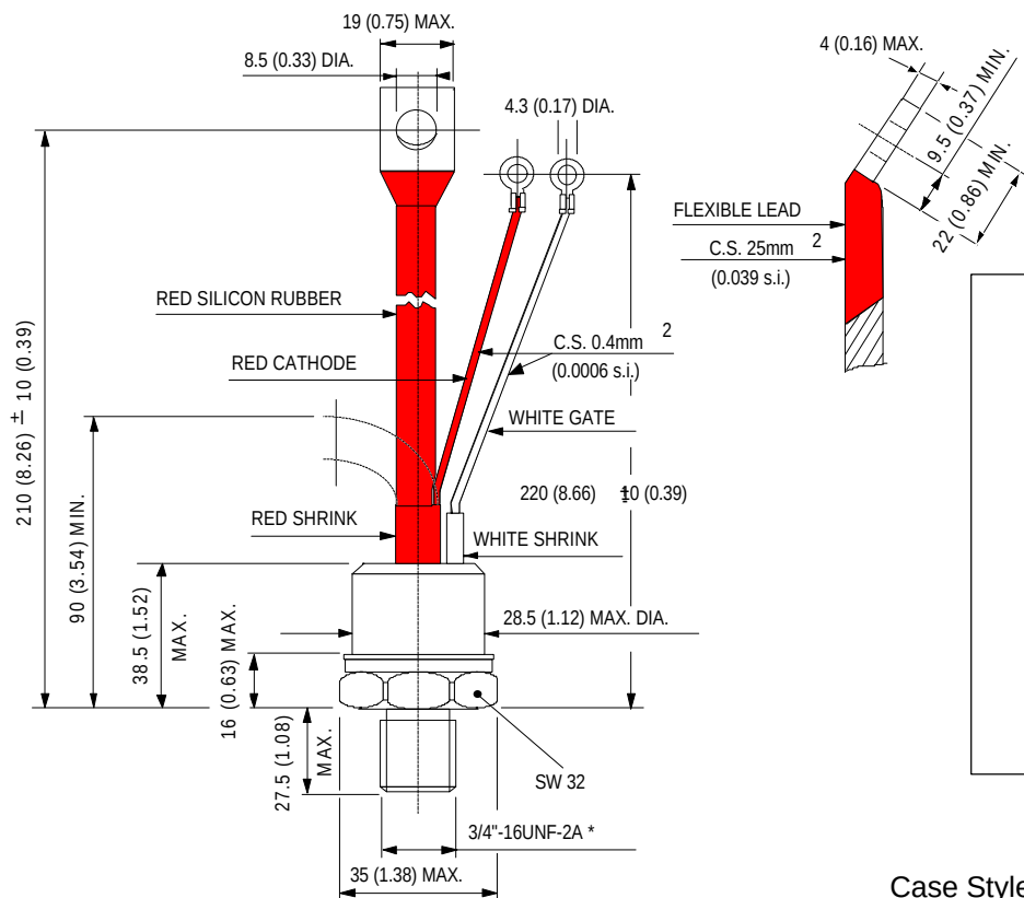
Case Style TO-209AB (TO-93) All dimensions in millimeters (inches)
