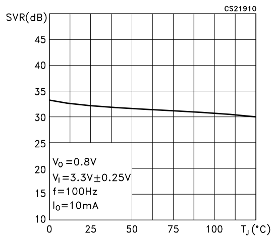
Figure 15: Supply Ripple Rejection vs Temperature
