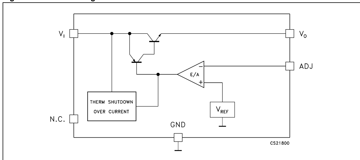
Figure 1: Schematic Diagram
