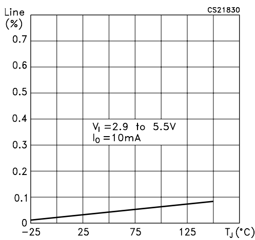
Figure 6: Line Regulation vs Temperature
