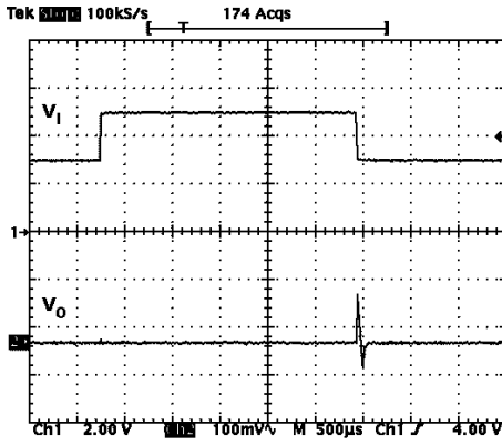
Figure 23: Line Transient
