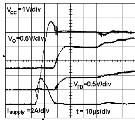
Figure 20: Start-Up Transient
