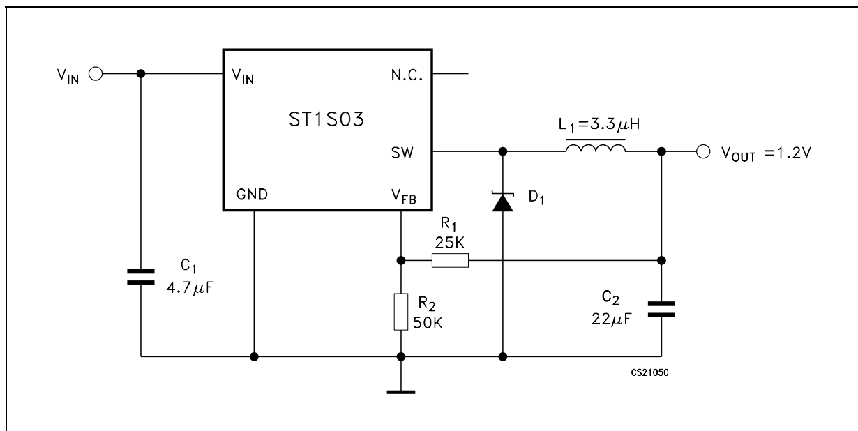
Figure 3: Application Circuit
