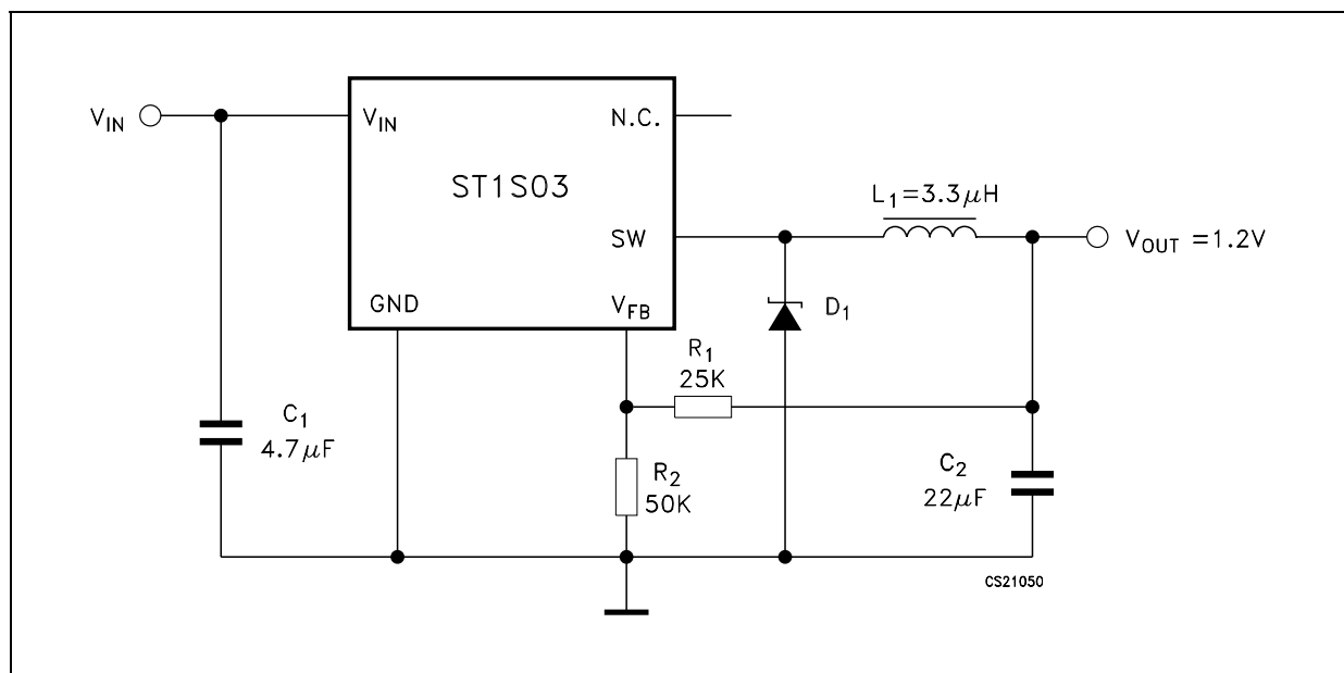
Figure 3: Application Circuit
