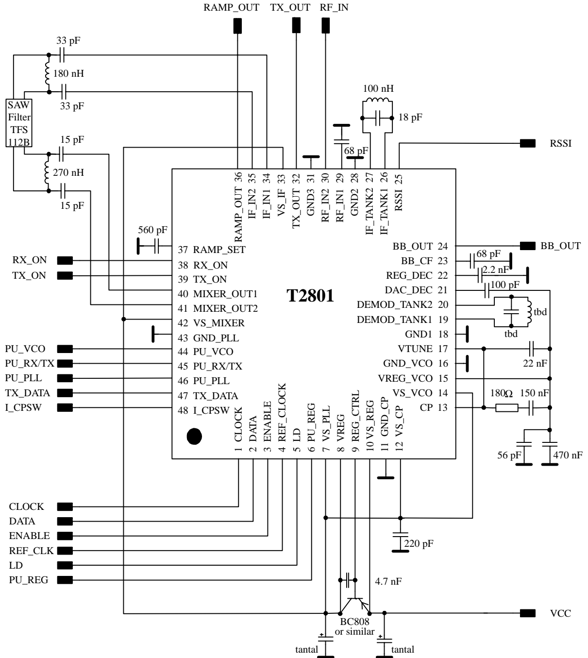
Figure 6. Application circuit
