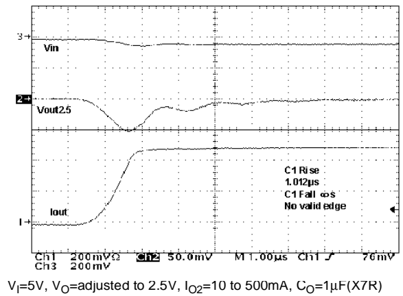
Figure 23 : Load Transient
