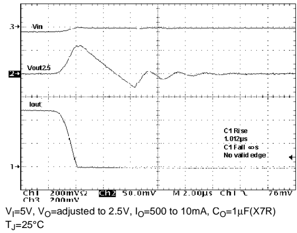
Figure 23 : Load Transient
