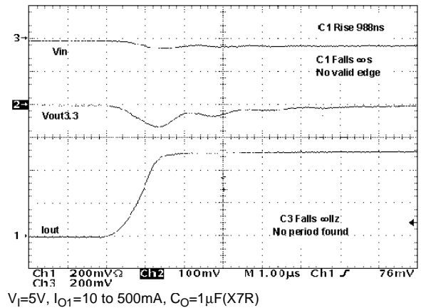
Figure 24 : Load Transient
