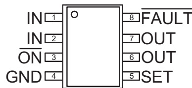
SOP-8/TSSOP-8 (Top View)
