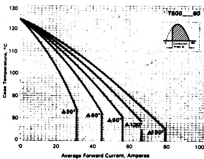
Maximum Case Temperature VS. Forward Current
