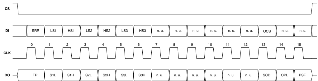
Figure 3. Data Transfer
