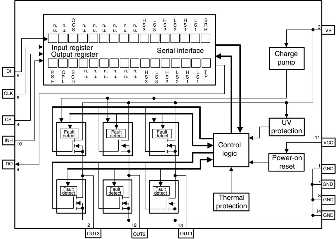
Figure 1. Block Diagram
