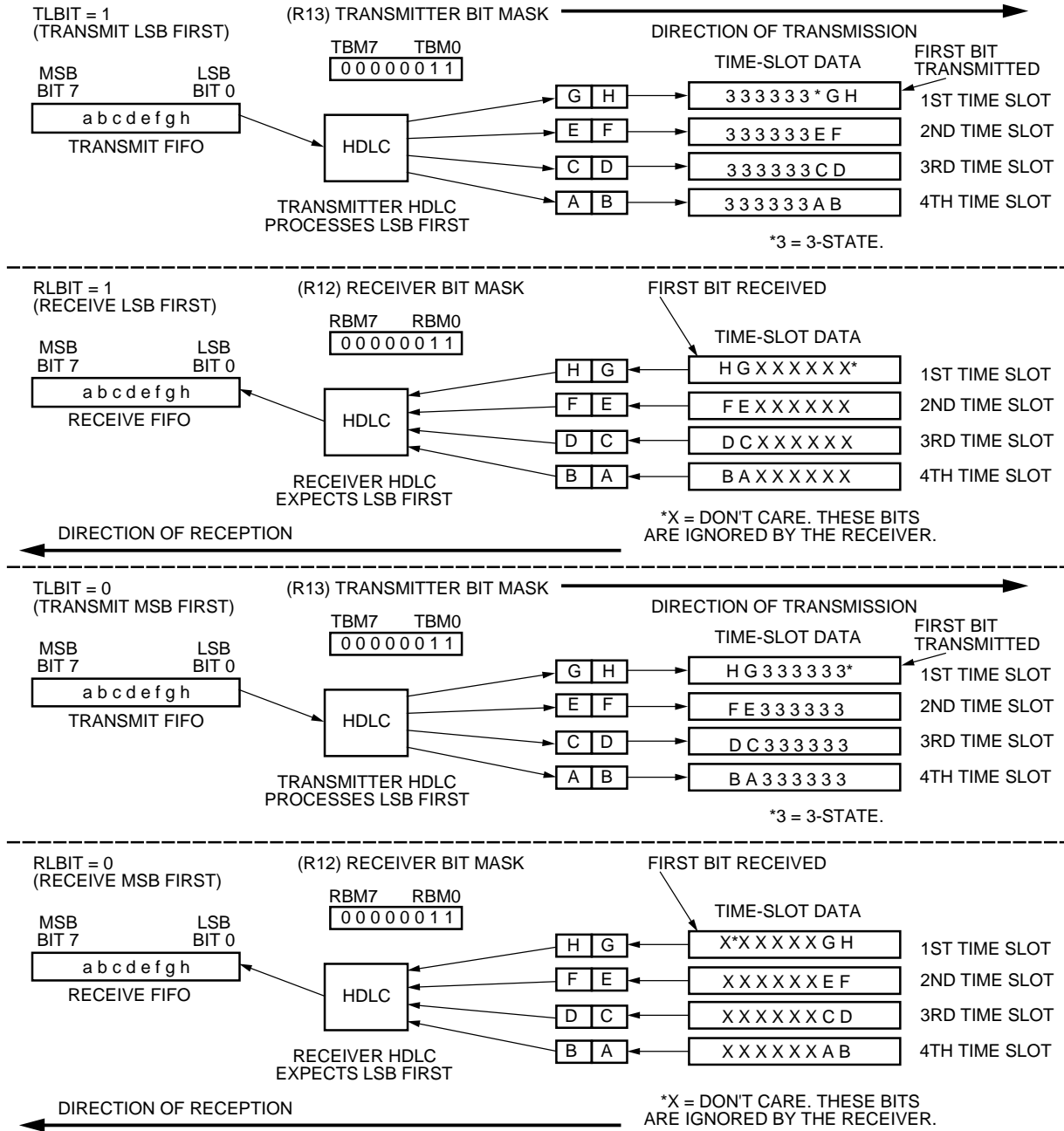
Figure 8. 16 kbits/s Operation
