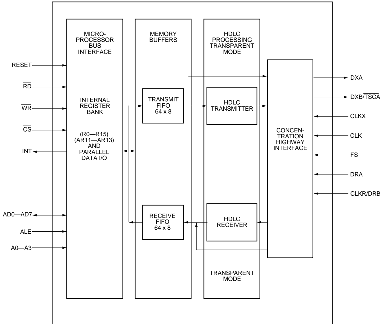
Figure 1. Block Diagram
