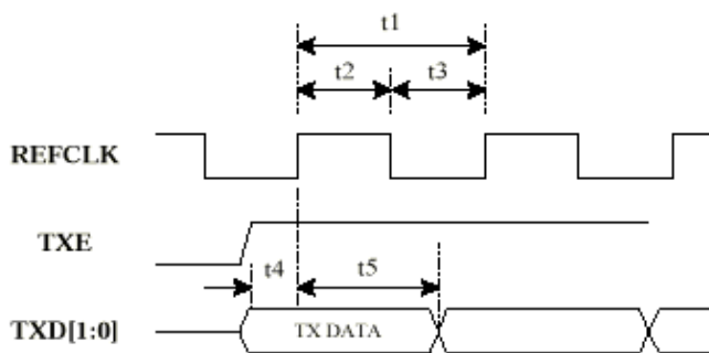
RMII Transmit Timing
