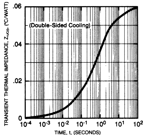
TRANSIENT THERMAL IMPEDANCE CHARACTERISTICS (JUNCTION TO CASE)
