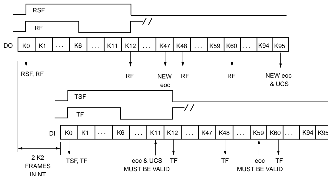
Figure 16. K2-to-U Mapping
