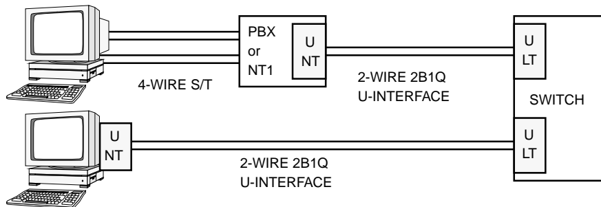
Figure 22. Loop Application
