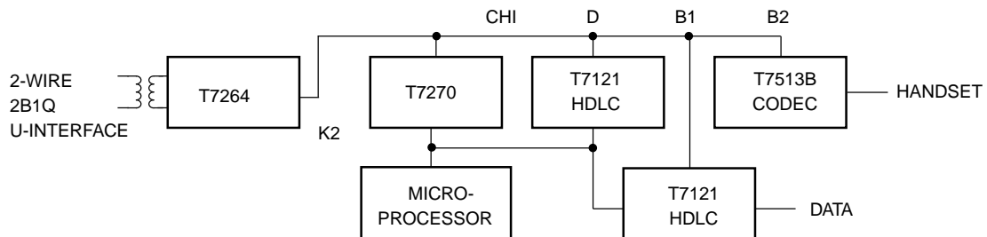
Figure 22. Loop Application
