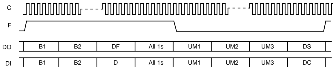
Figure 9. K2 Octets
