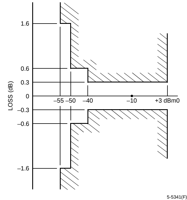
Figure 7. Loss vs. Level
