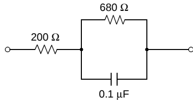
Figure 5. Termination Impedance
