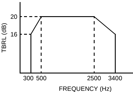
Figure 9. Hybrid Balance
