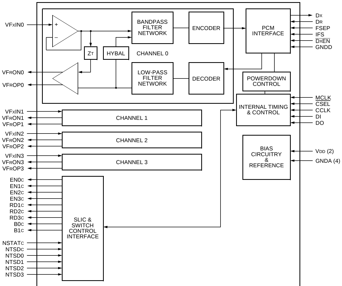
Figure 1. Block Diagram
