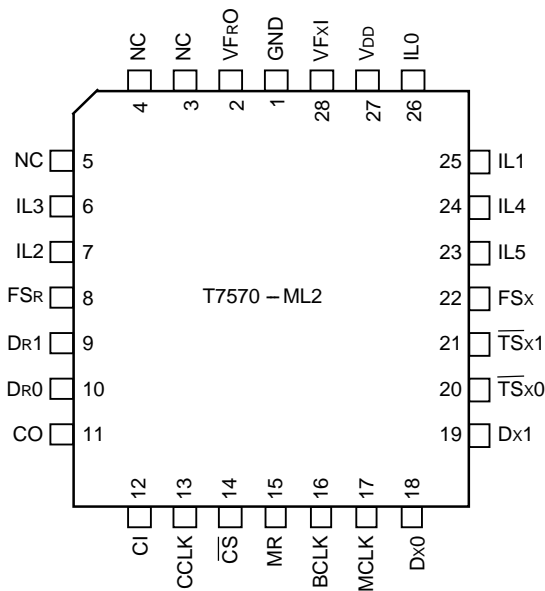
Figure 2. Pin Diagram
