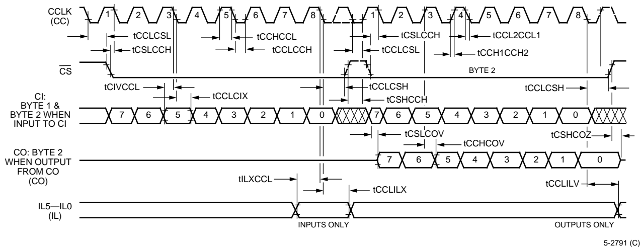
Figure 6. Serial Control Port Timing
