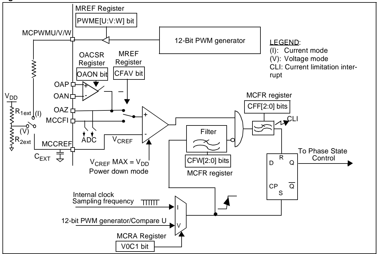
Figure 104. Current Feedback
