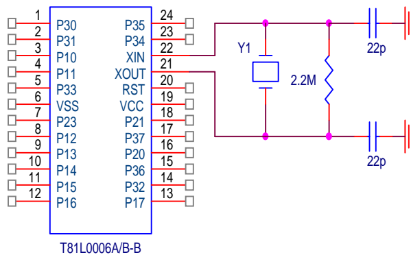
Crystal Oscillator
