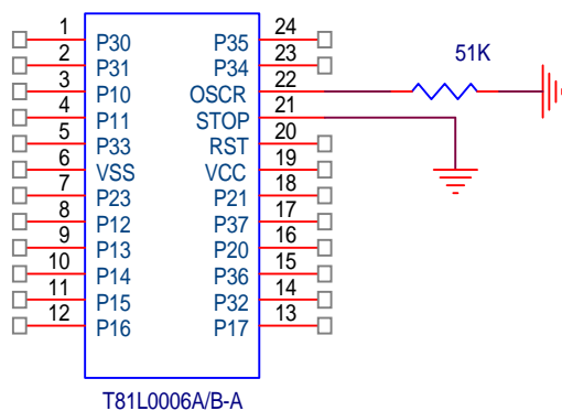
RC Oscillator
