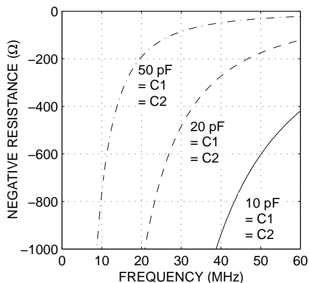
Figure 20. Negative Resistance Plot
