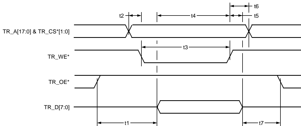
Figure 28. External LUT Memory Write Timing (cyc_per_acc = 2 and cyc_per_acc = 3)
