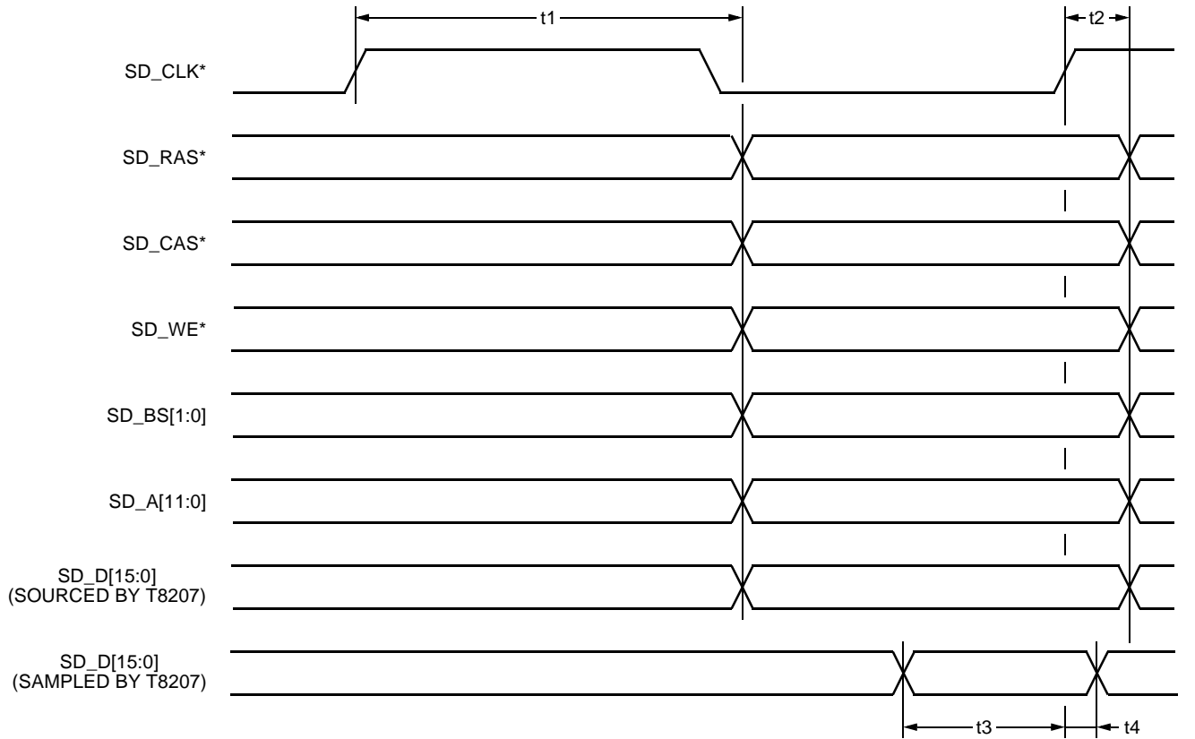
Figure 30. SDRAM Interface Timing
