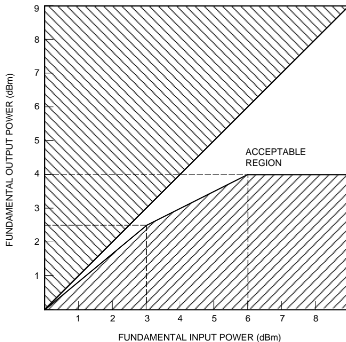
Figure 4. Overload Compression
