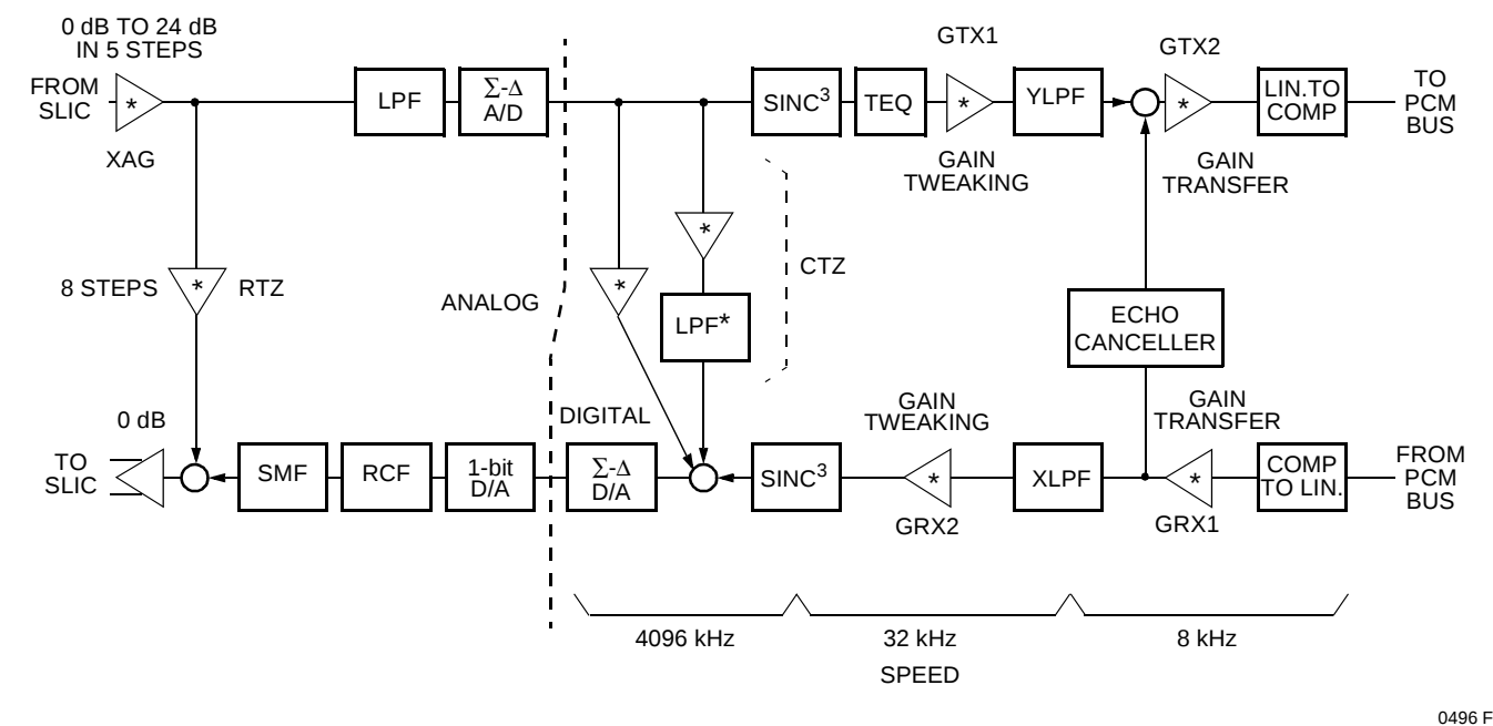
Figure 20. Internal Signal Processing
