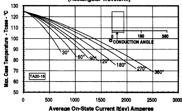
Maximum Allowable Case Temperature
