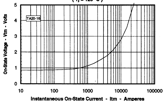
Maximum On-State Forward Voltage Drop
