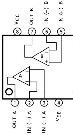
TA75557F
