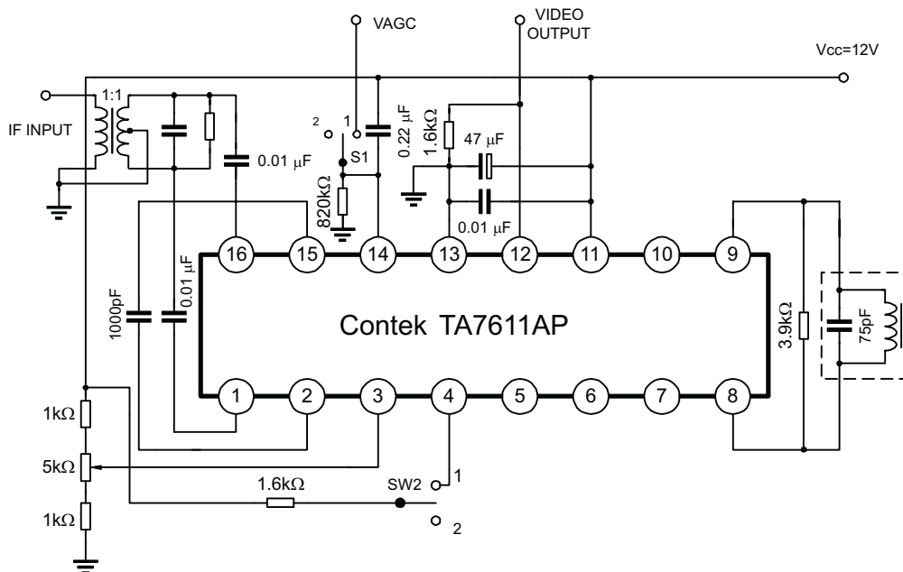
TEST CIRCUIT 2
