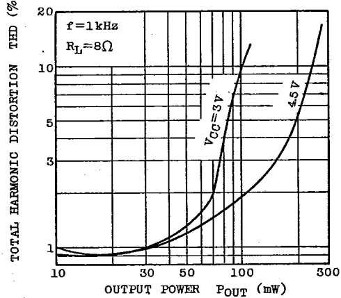
THD - P_{OUT}
