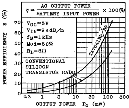
\eta - P_o CHARACTERISTIC COMPARISON
