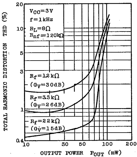
THD - P_{OUT}
