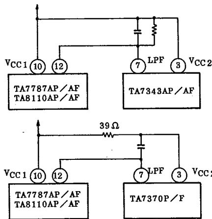
Fig.4 CONNECTION TO TA7343AP/AF AND TA7370P/F
