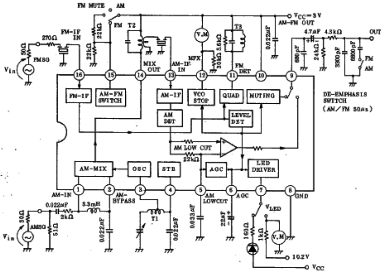
TEST CIRCUIT 1
