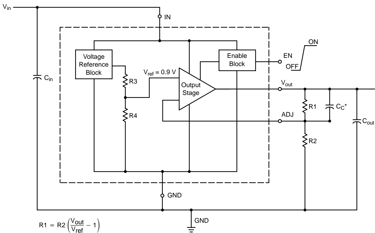
Figure 1. Typical Schematic, Adjustable Output Version
