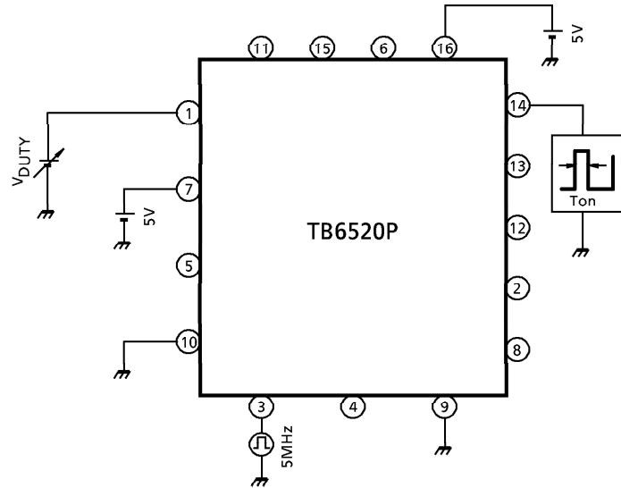
TEST CIRCUIT 9: V_{AD}(L) , V_{AD}(H)
