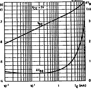
Fig. 3 - Input voltage and input offset voltage vs. emitter current
