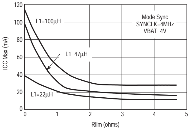
Figure 8. Maximum Card Supply Current vs. R LIM (V CC =5V, V BAT =4V)
