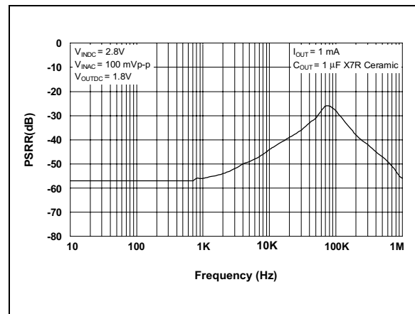
FIGURE 4-18: Power Supply Rejection Ratio vs. Frequency.
