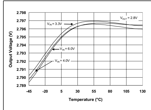
FIGURE 4-16: Output Voltage vs. Temperature.
