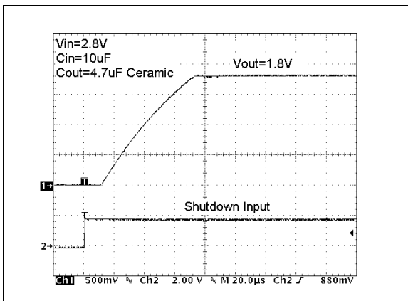
FIGURE 4-21: Wake-Up Response.
