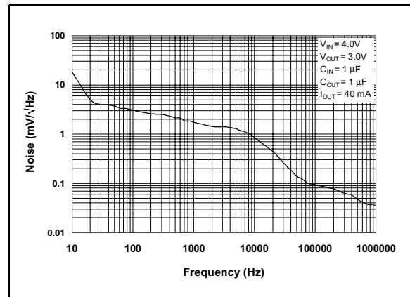
FIGURE 4-17: Output Noise vs. Frequency.
