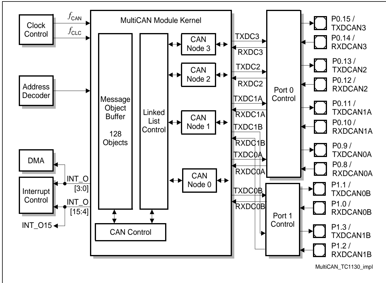
Figure 12 General Block Diagram of the MultiCAN Interfaces
