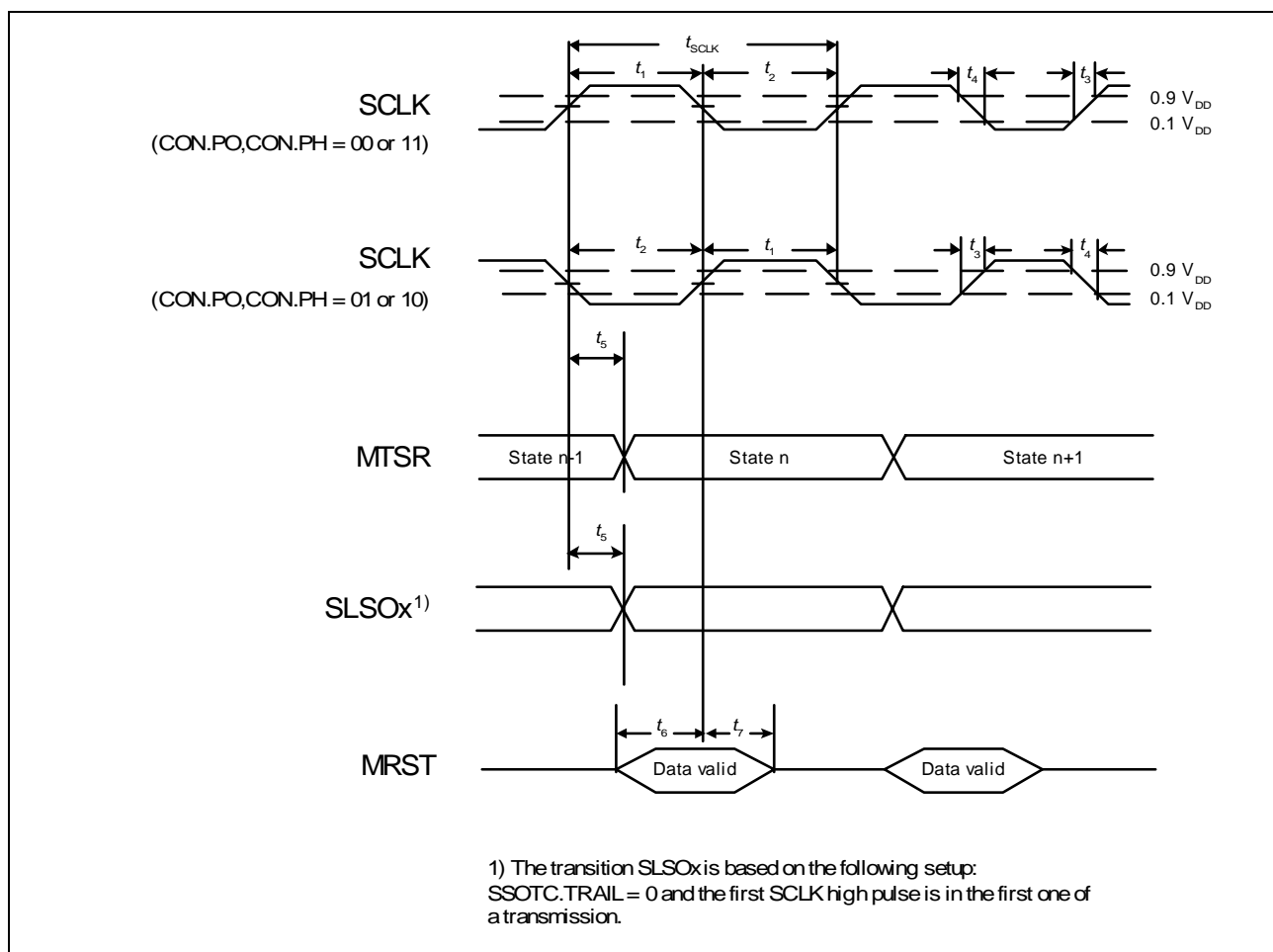
Figure 34 SSC Master Mode Timing
