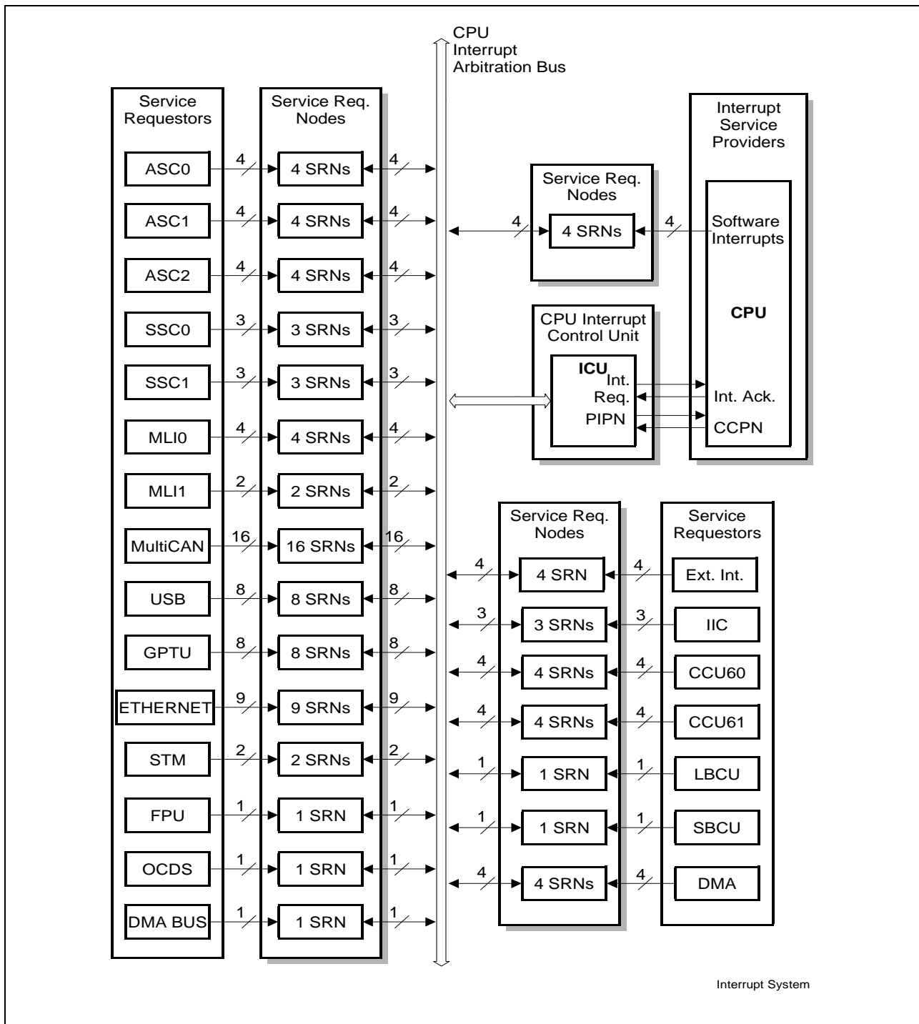
Figure 17 Block Diagram of the TC1130 Interrupt System
