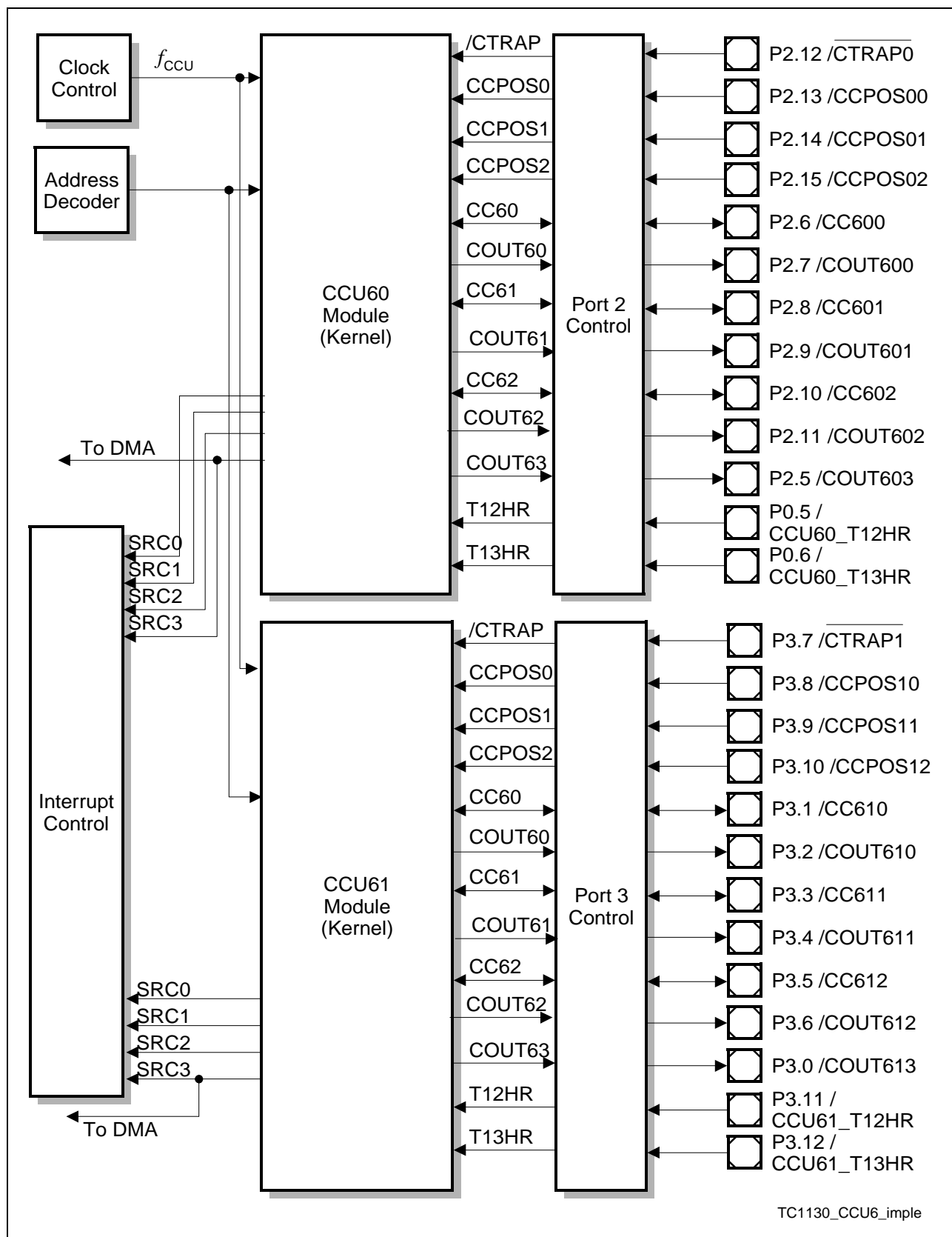
Figure 11 General Block Diagram of the CCU6
