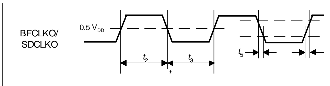
Figure 27 EBU Clock Output Timing
