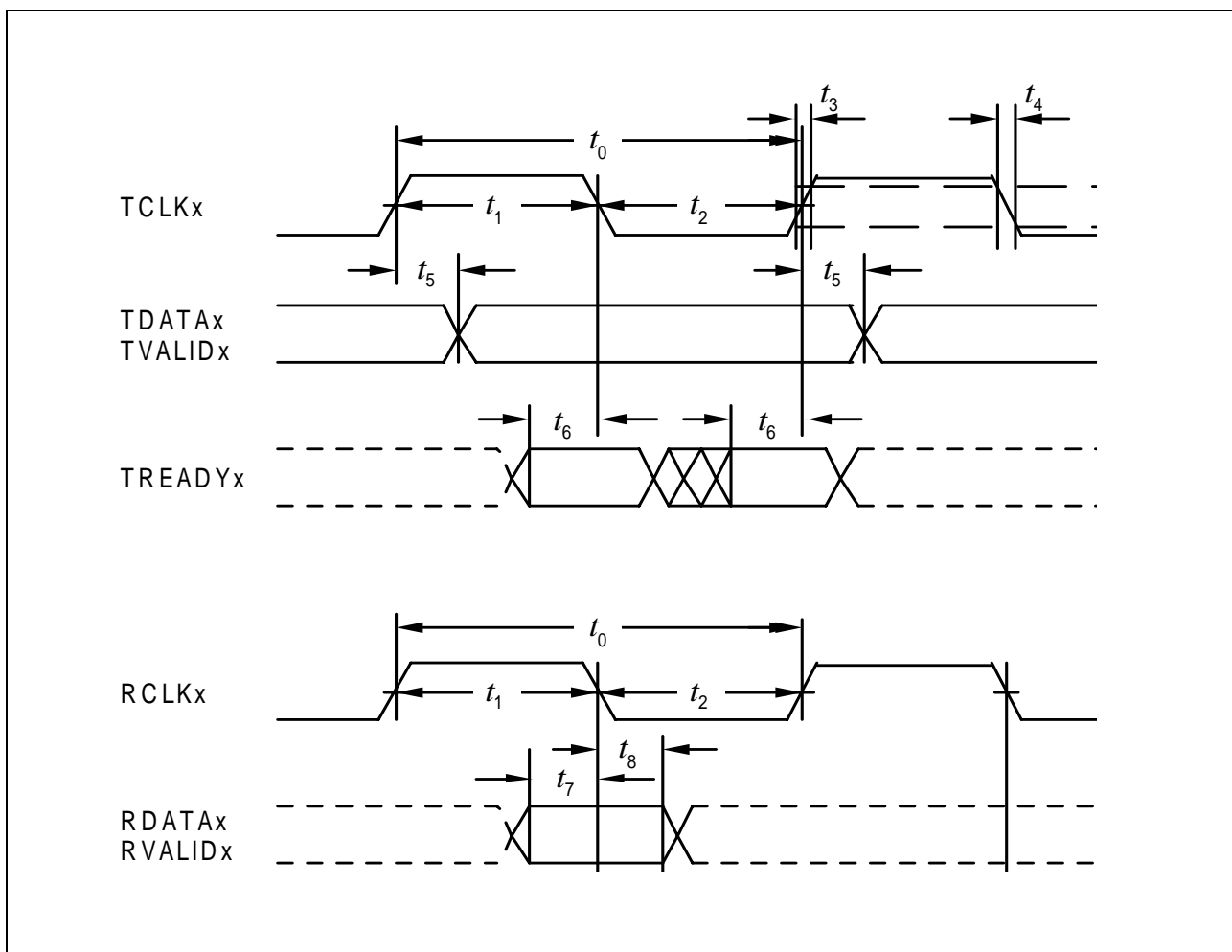
Figure 35 MLI Interface Timing
