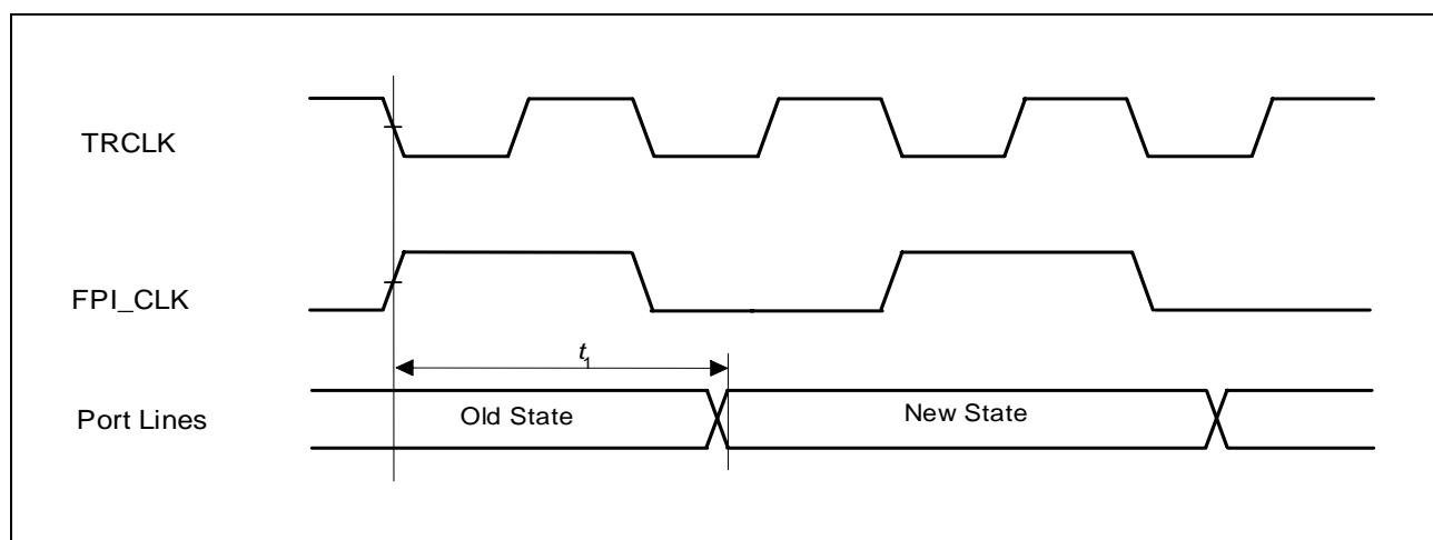
Figure 26 Port Timing
