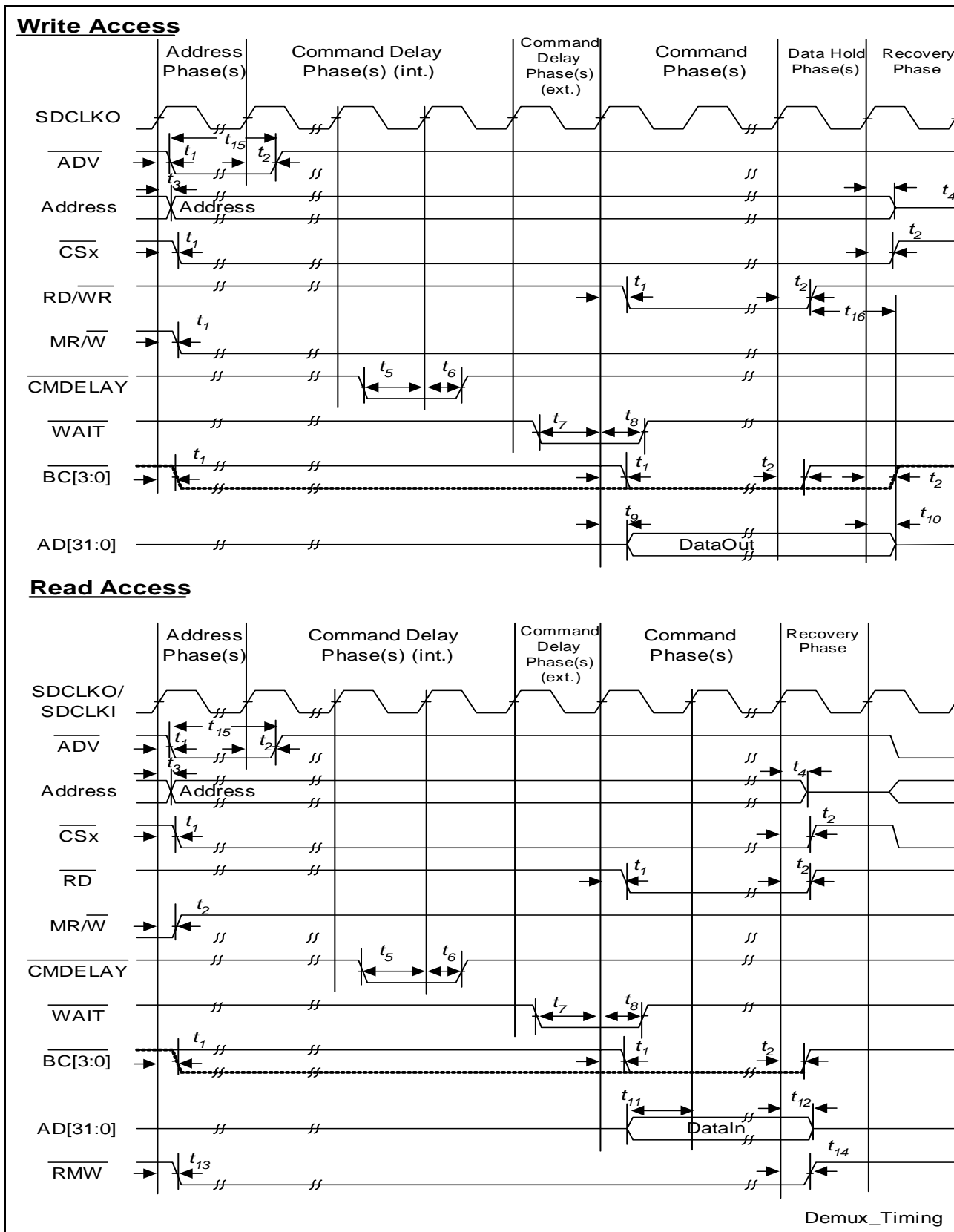
Figure 30 Demultiplexed Asynchronous Device Access Timing
