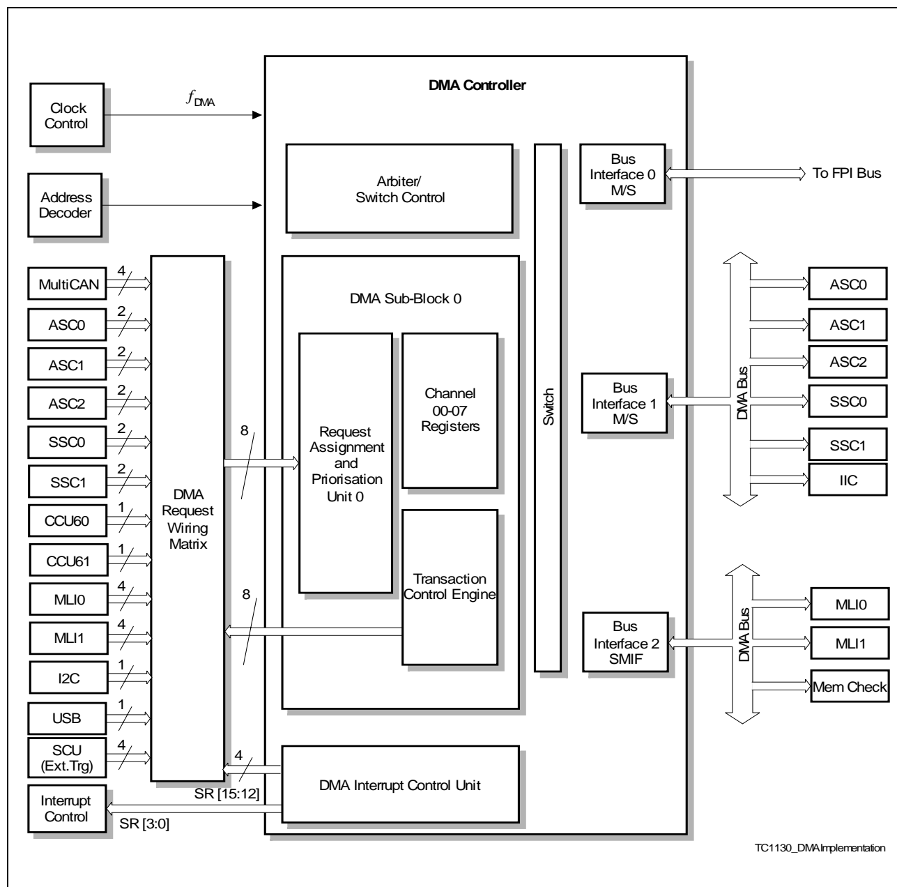
Figure 15 DMA Controller Structure and Interconnections
