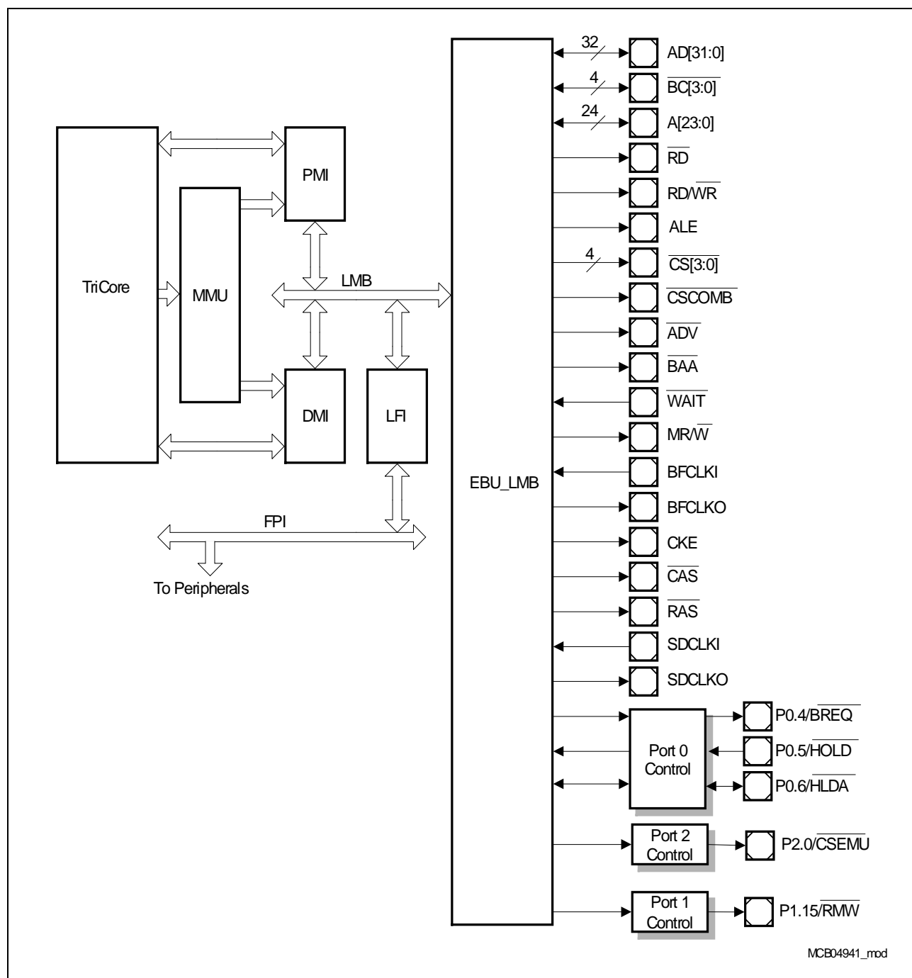
Figure 14 EBU Structure and Interfaces
