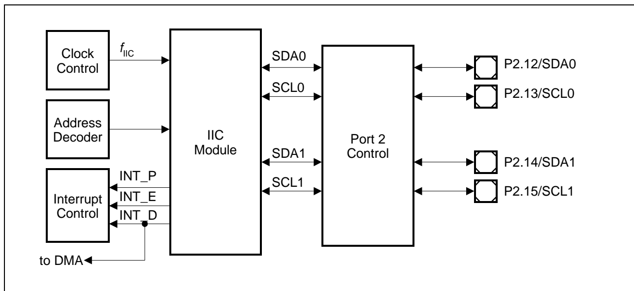
Figure 7 General Block Diagram of the IIC Interface
