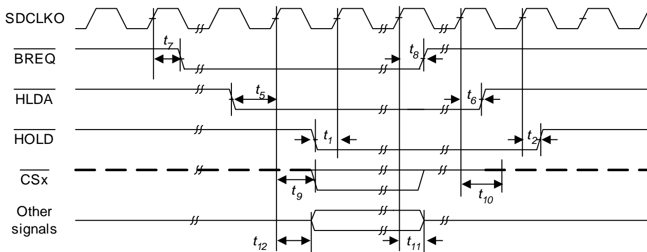
Figure 32 External Bus Arbitration Timing
