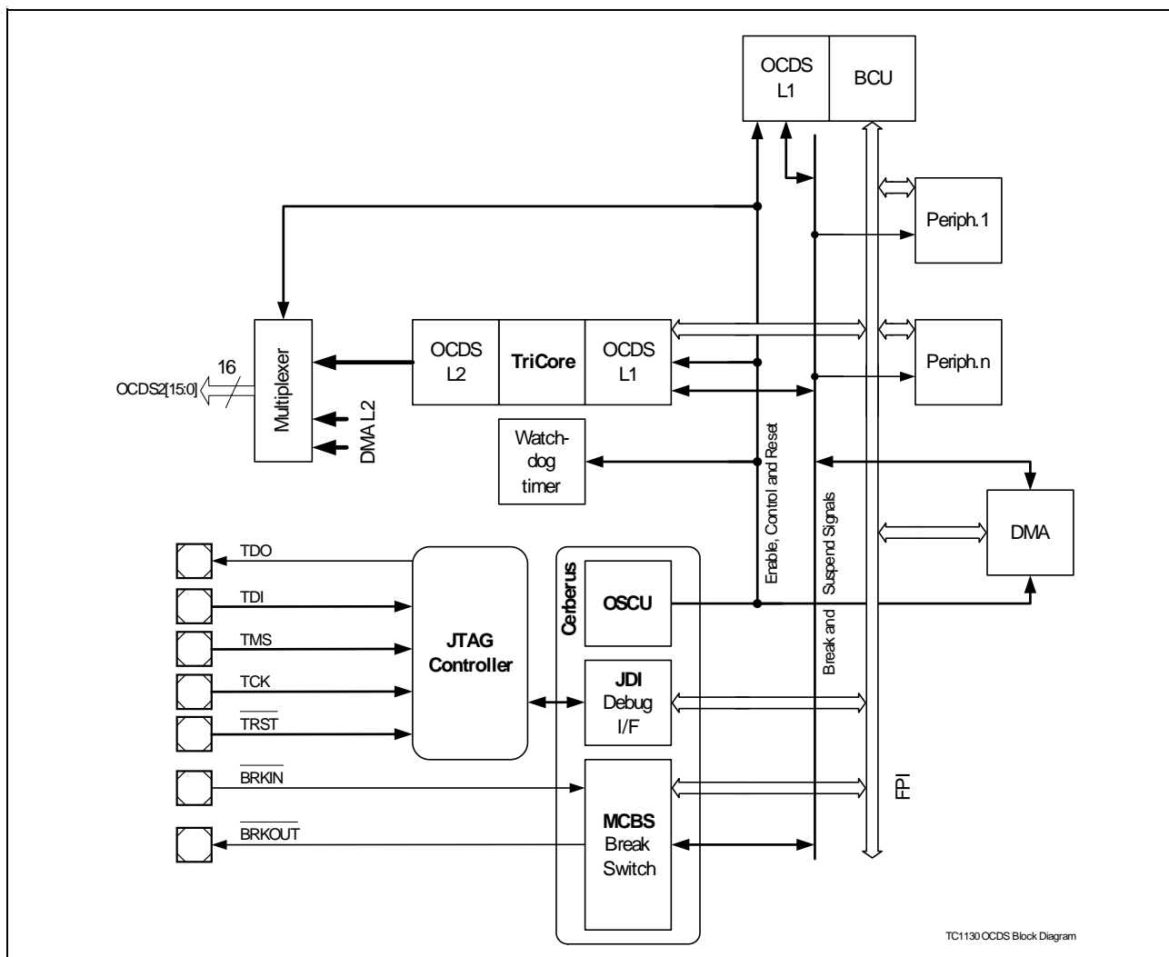
Figure 18 OCDS Support Basic Block Diagram
