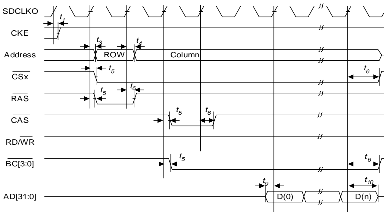
Figure 28 SDRAM Access Timing
