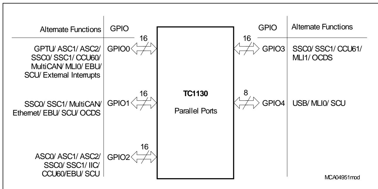
Figure 4 Parallel Ports of the TC1130
