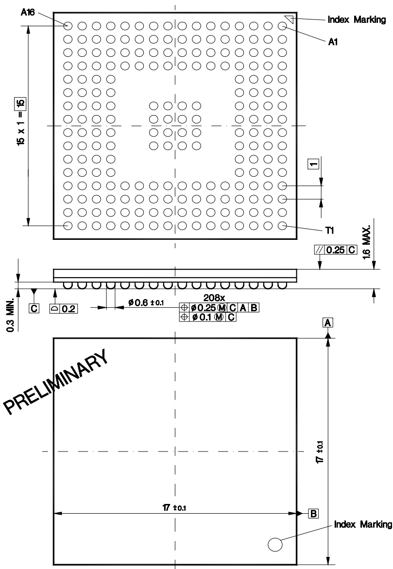
Figure 40 P-LBGA-208-2 Package
