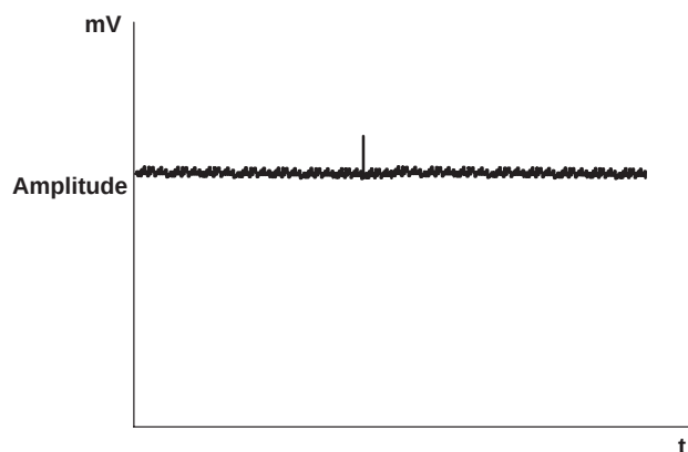
Figure 11. Pixel Nonuniformity, Dark Condition
