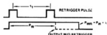
TYPICAL I/O PULSES CONTROL UTILIZING RETRIGGER PULSE
