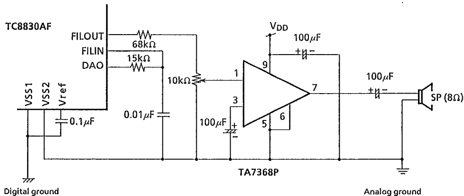
Fig.5.45 Connection of audio amplifier
