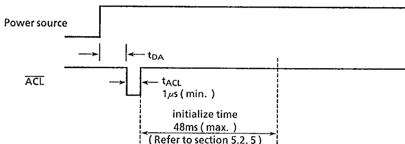
Fig.5.29 \overline{ACL} pulse width
