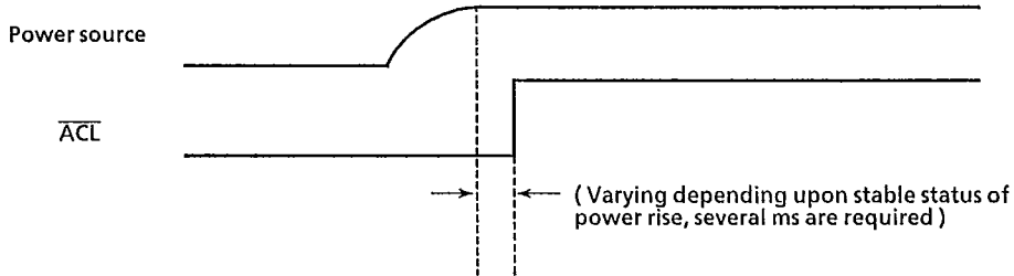
Fig. 5.32 System initialization by CPU control
