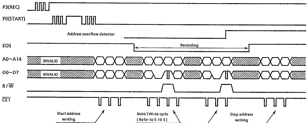
Fig. 5.33 Recording at manual control
