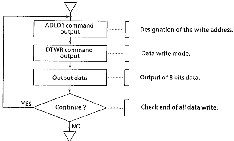
Fig.5.20 Data write procedure
