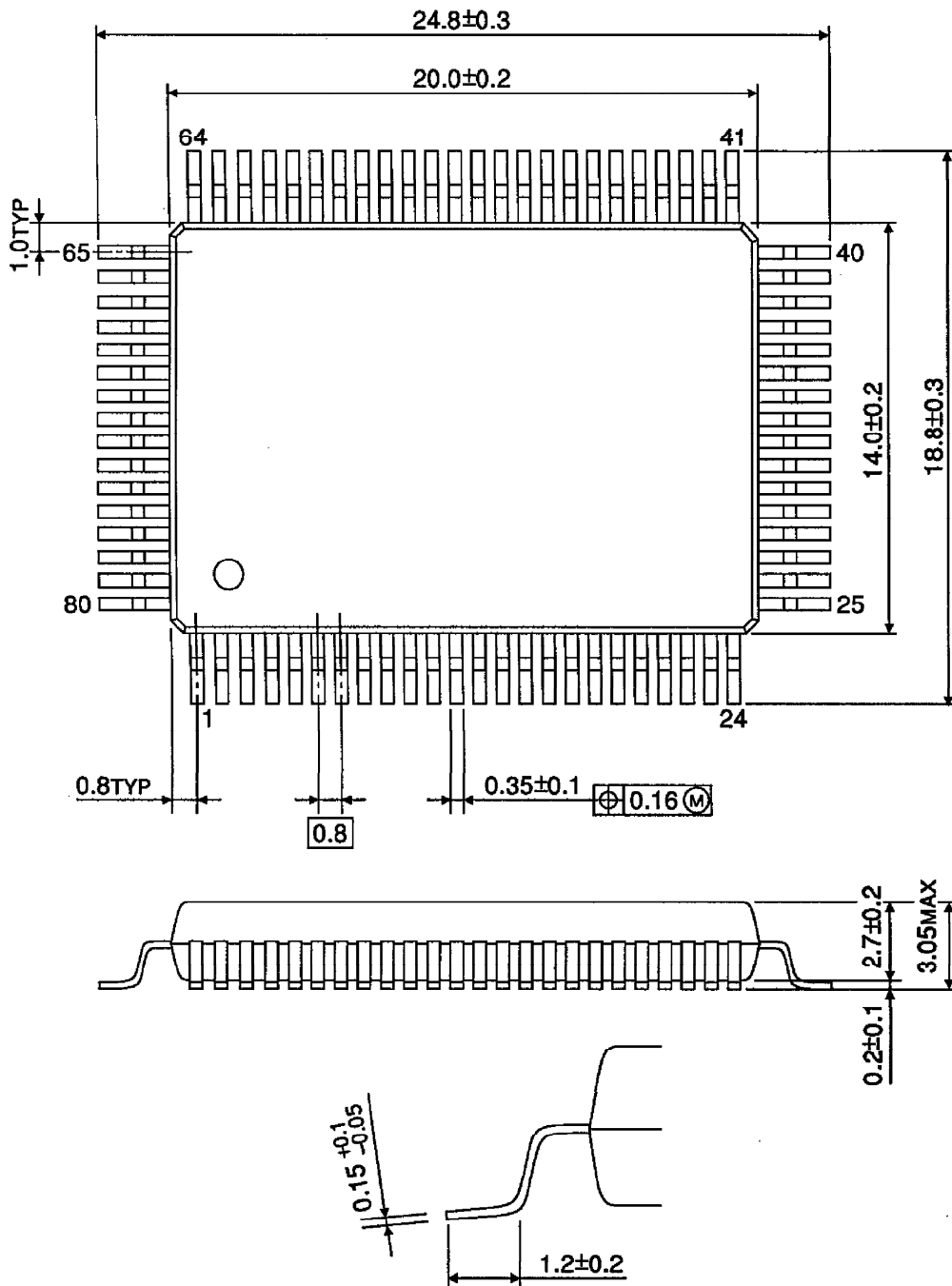
OUTLINE DRAWING QFP80-P-1420-0.80A
