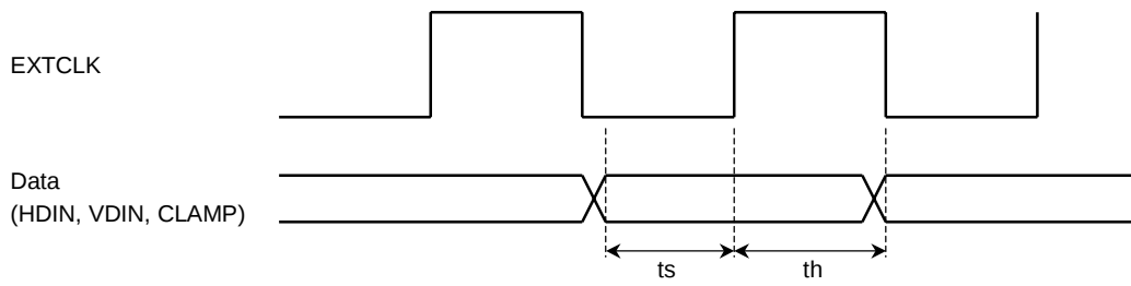
Figure 6 Data Set-up Hold Time
