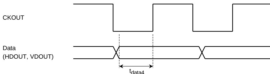
Figure 7 Phase Difference between Clock and Data Output
