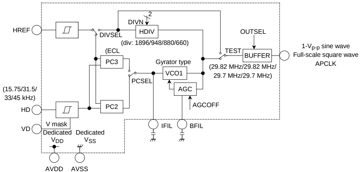
Figure 5 Block Diagram of HPLL
