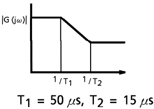
Fig.5 Filter Characteristics
