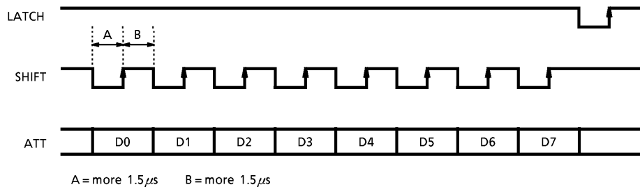
FIG.13 Example for serial control mode data
